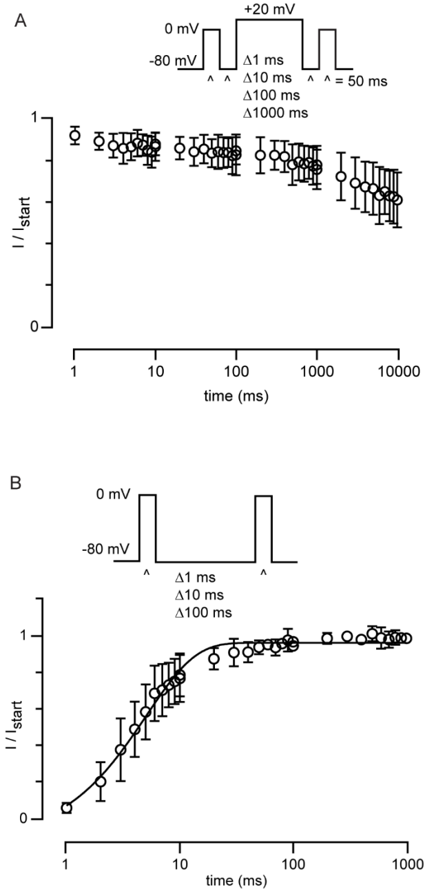
Supplemental Figure 7. Fast and slow inactivation kinetics of hNav1.8 in HEK293 cells
